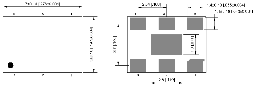
External Dimensions
