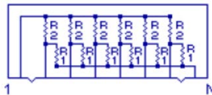
Dual Terminator SRT [Schematic 5]
