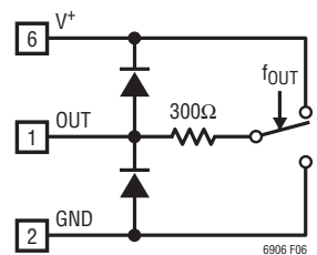
Figure 6. OUT Pin
