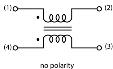
Equivalent circuit
