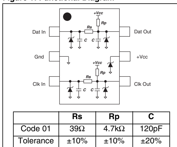
Figure 1: Functional Diagram
