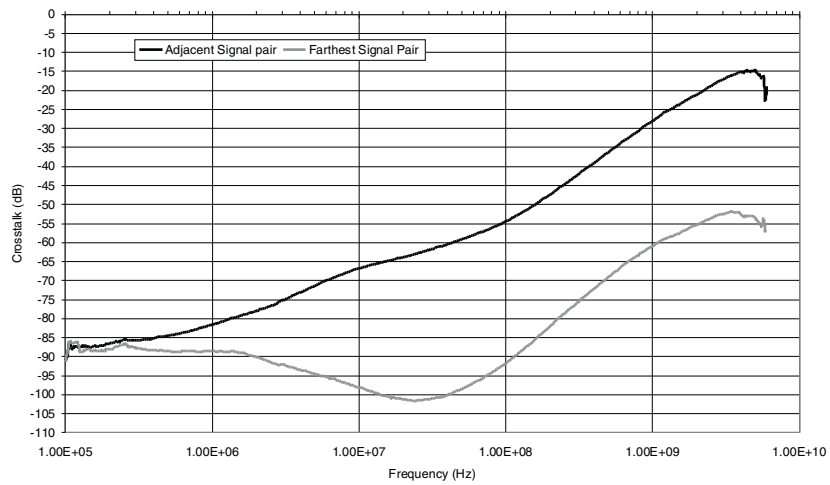
Figure 9. TPD8F003
