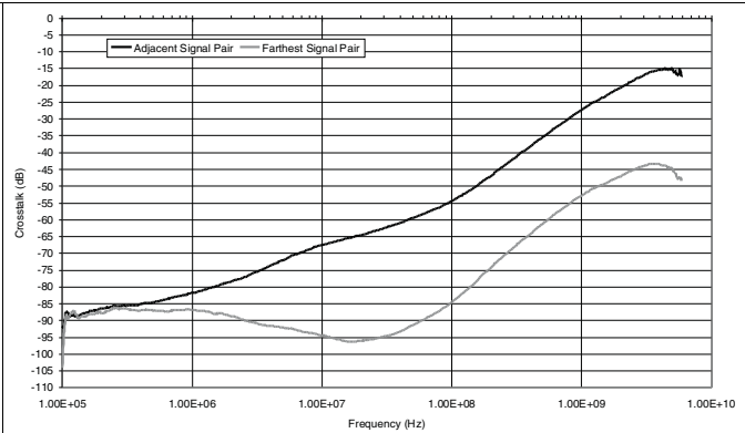
Figure 8. TPD6F003
