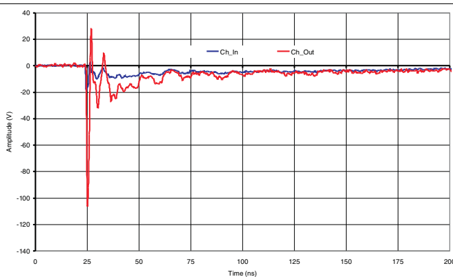
Figure 4. With -12 kV Contact ESD Stress at Ch_Out
