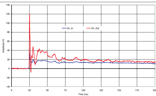
Figure 2. With 12 kV Contact ESD Stress at Ch_Out
