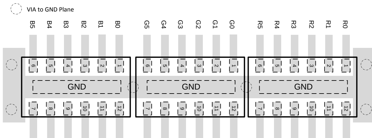
Figure 12. TPD6F003 Layout
