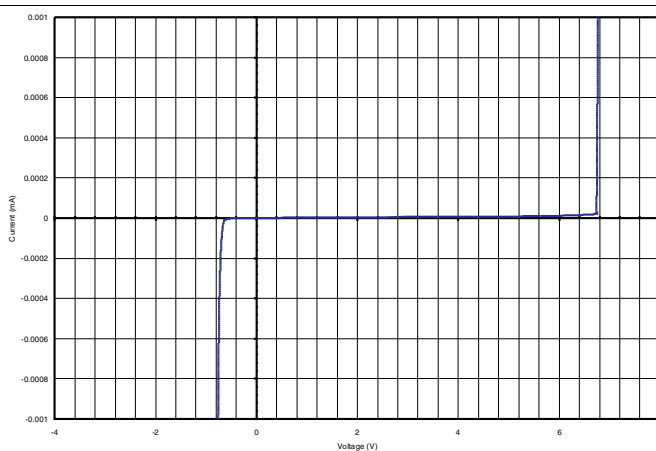
Figure 6. DC Voltage-Current Sweep Across Input/Output Pins
