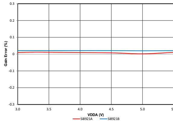
Figure 28. Gain Error (%) vs. VDDA Supply (V)
