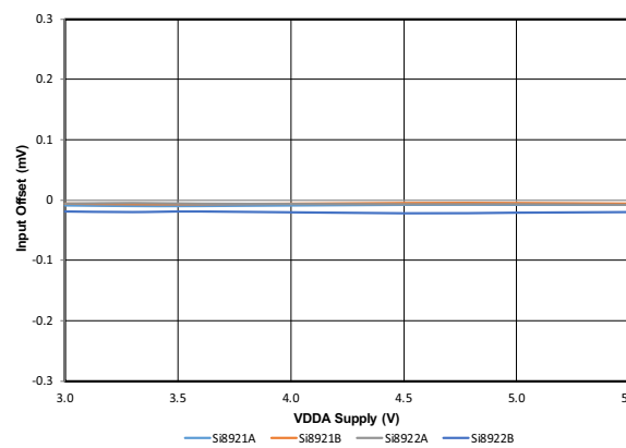
Figure 26. Input Offset (mV) vs. VDDA Supply (V)
