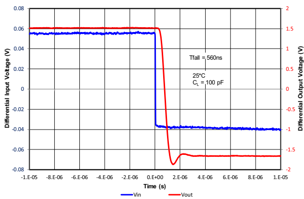
Figure 35. Si8921A High-to-Low Step Response
