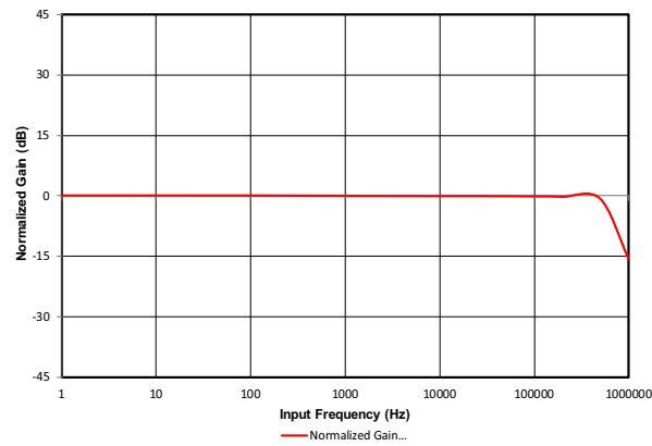
Figure 29. Amplifier Bandwidth
