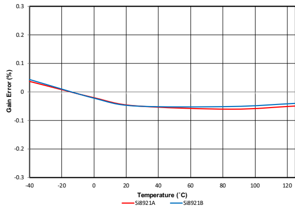
Figure 27. Gain Error (%) vs. Temperature (°C)
