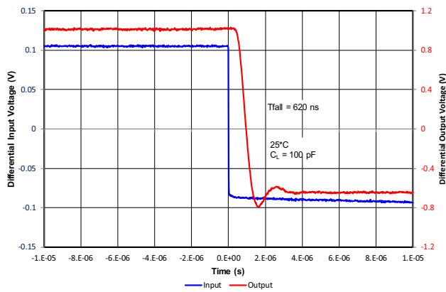
Figure 33. Si8921B High-to-Low Step Response
