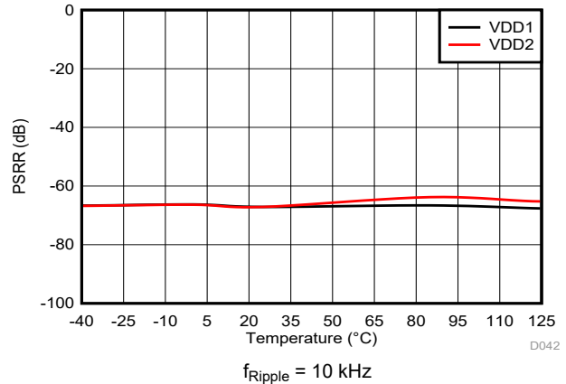
Figure 6-32. Power-Supply Rejection Ratio vs Temperature
