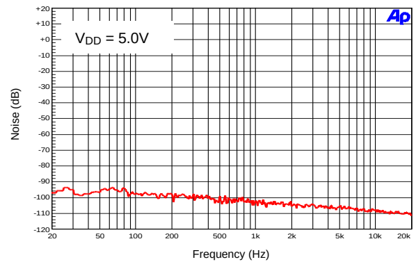
Noise Floor
