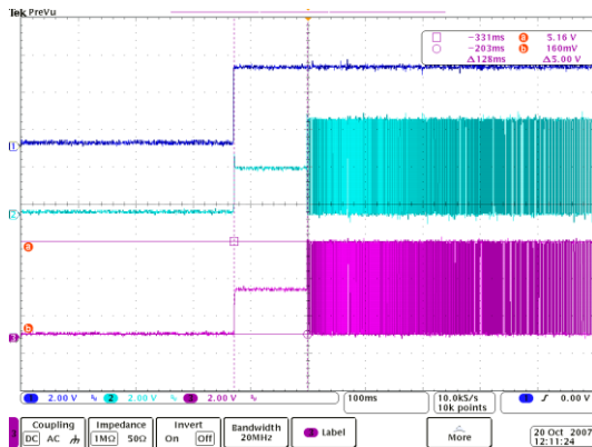
Startup Response
