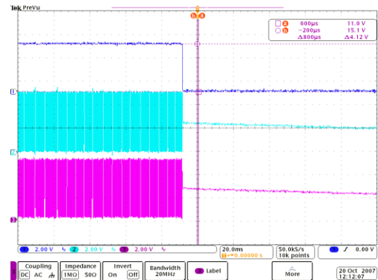
Shutdown Response
