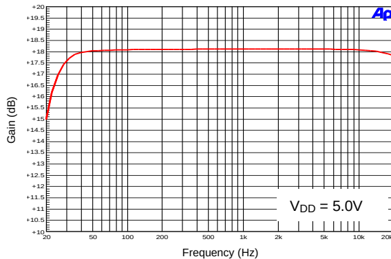
Frequency Response
