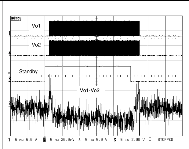
Figure 55. Startup and shutdown times V_{CC} = 5V, G = 6dB, C_{in} = 1\mu F (5ms/div)
