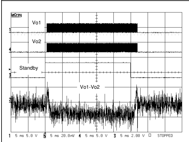
Figure 56. Startup and shutdown times V_{CC} = 3V, G = 6dB, C_{in} = 1\mu F (5ms/div)
