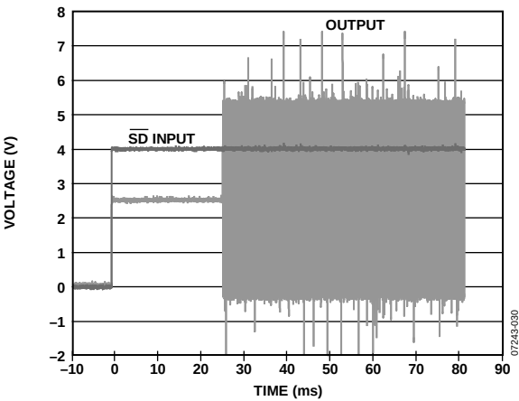
Figure 30. Turn-On Response
