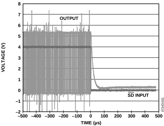
Figure 31. Turn-Off Response
