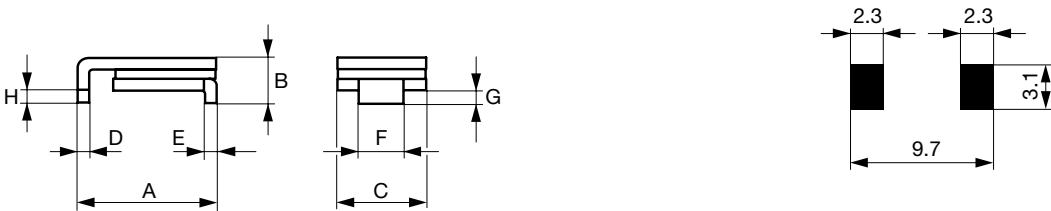
Solder pads PFSM.030.2 - PFSM.125.2 and PFSM.260.2
