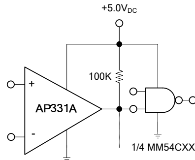
Driving CMOS
