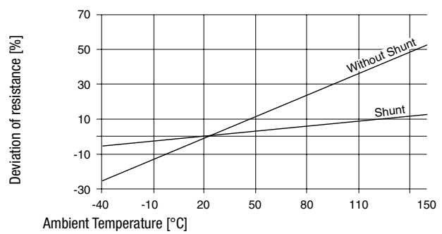
Derating Curve with Shunt (RTS-AS500)
