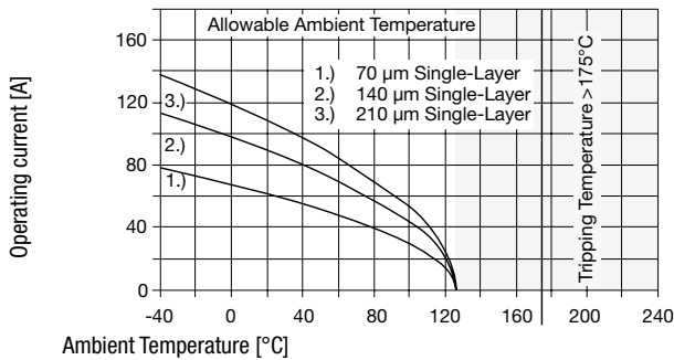
Derating Curve without Shunt (RTS-AC100)
