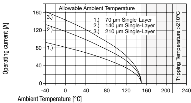
Derating Curve without Shunt (RTS-AC100)
