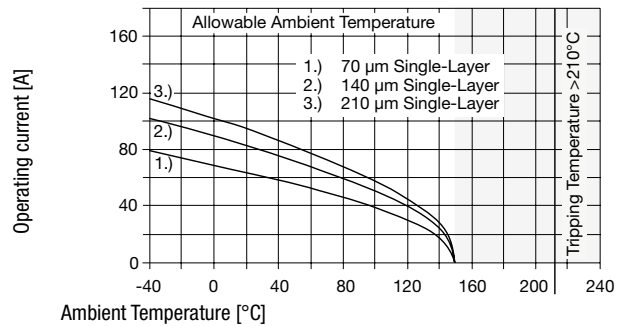
Derating Curve with Shunt (RTS-AS500)
