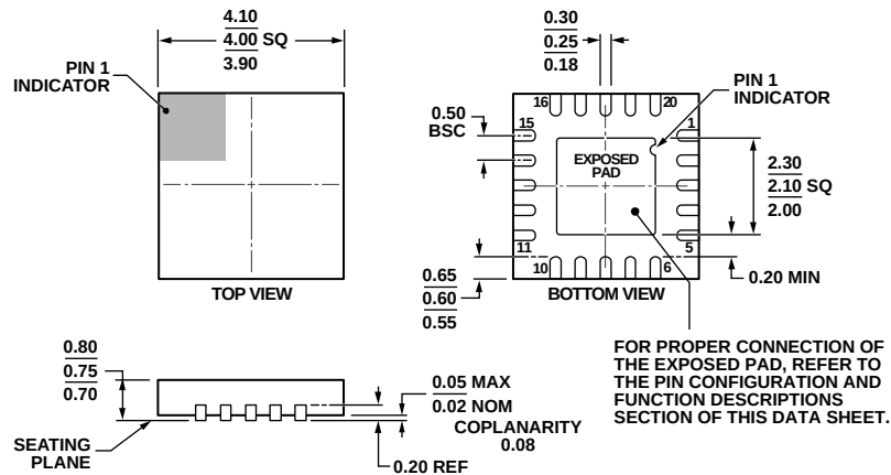
Figure 26. 20-Lead Lead Frame Chip Scale Package [LFCSP_WQ] 4 mm x 4 mm Body, Very Very Thin Quad (CP-20-6) Dimensions shown in millimeters
