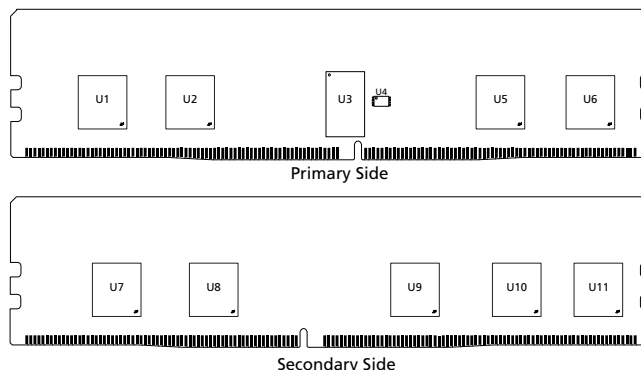
Figure 1: 288-Pin RDIMM
