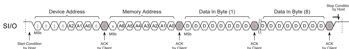
Figure 7-2. Page Write
