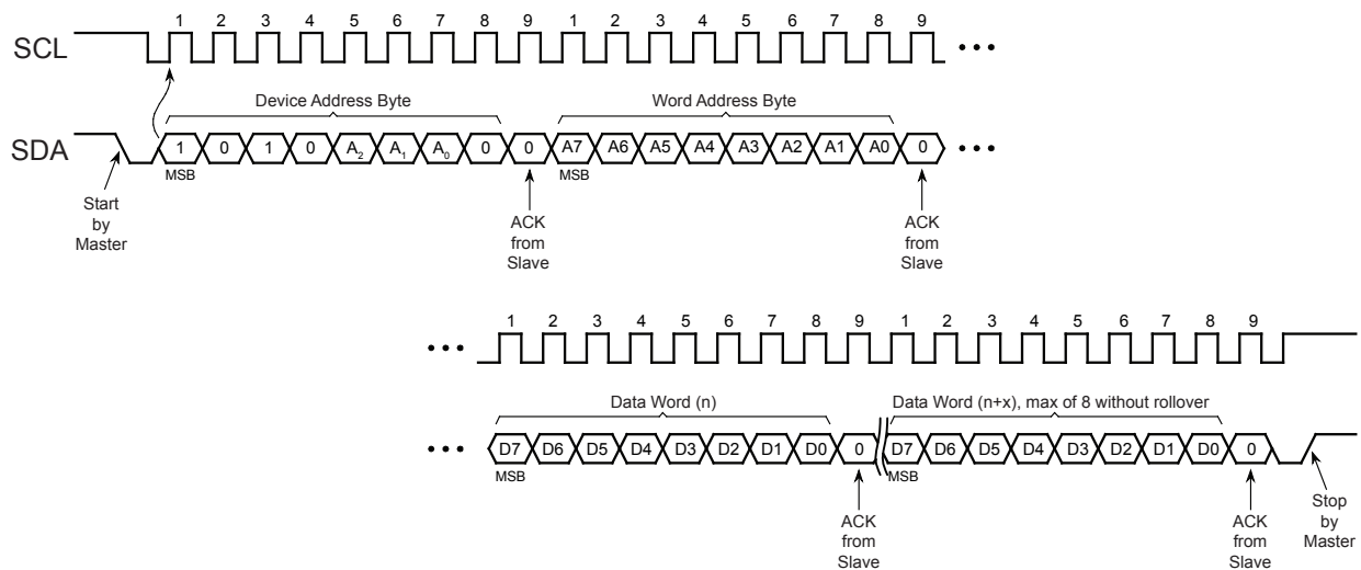
Figure 7-2. Page Write
