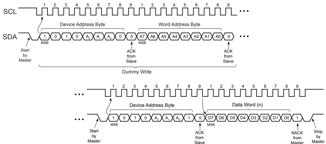
Figure 8-2. Random Read
