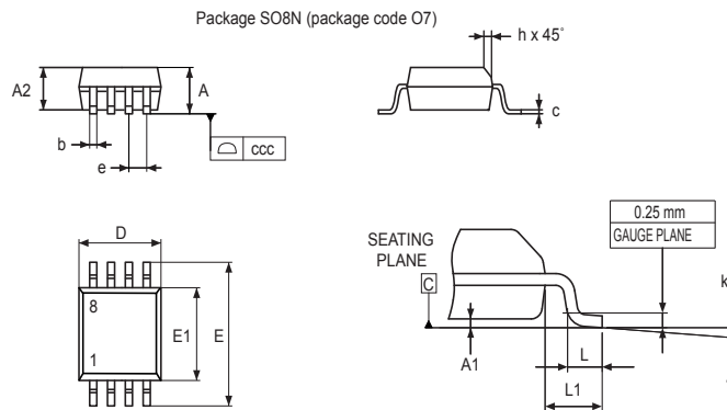
Figure 23. SO8N – Outline
