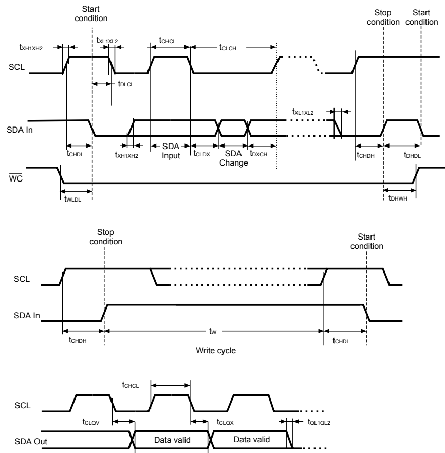
Figure 14. AC waveforms
