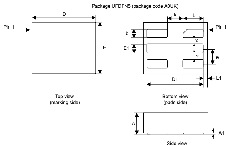
Figure 17. UFDFPN5 - Outline
