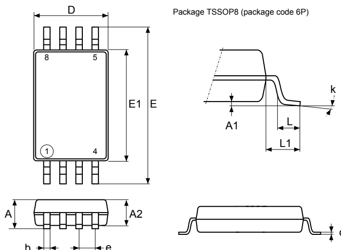
Figure 21. TSSOP8 – Outline
