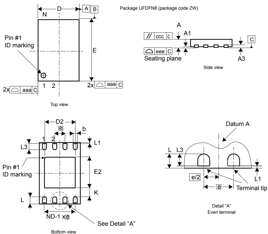
Figure 19. UFDFPN8 - Outline
