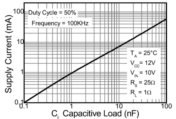
Supply Current
