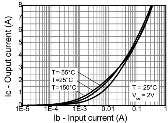
Sink Current Vs Input Current
