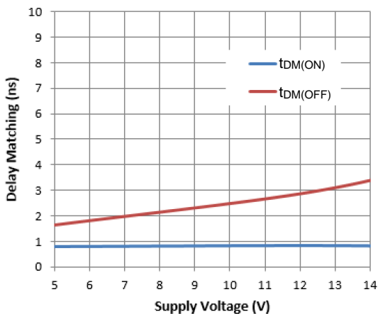
Figure 15. Delay Matching vs. Supply Voltage
