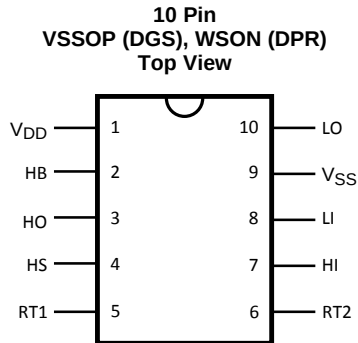
Pin Functions
