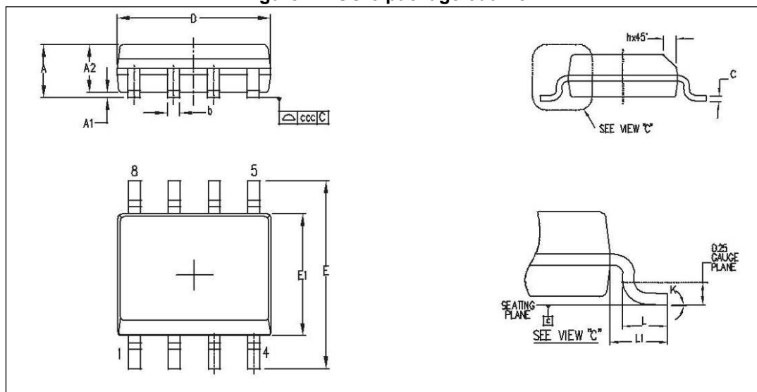
Figure 12. SO-8 package outline
