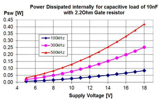
Figure 7. Power dissipation with load of 10 nF and 2.2 \Omega gate resistor
