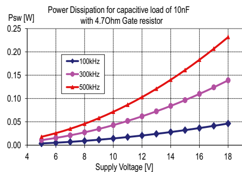
Figure 8. Power dissipation for capacitive load of 10 nF with 4.7 \Omega gate resistor
