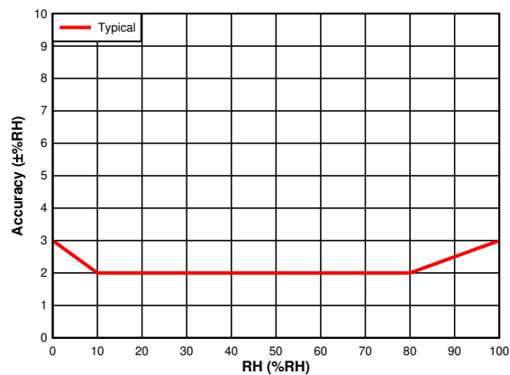
Figure 7-2. RH Accuracy vs. RH Set Point
