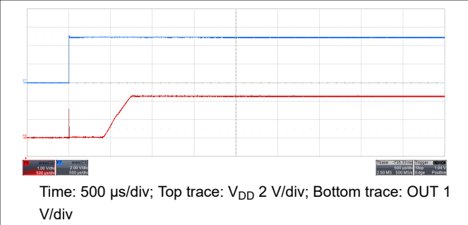
Figure 9-7. Output Turnon Response Time With a 1.1-nF Capacitive Load and V_{\text{DD}} = 5 \text{ V}
