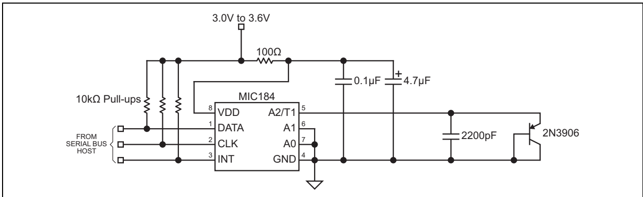
FIGURE 6-2: V_{DD} Decoupling for Very Noisy Supplies.
