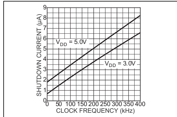
FIGURE 2-4: Shutdown I_{DD} vs. Frequency.
