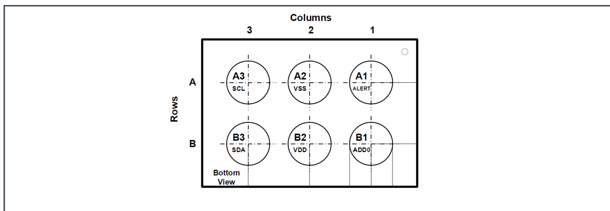
Figure 3: Pin Assignment WLCSP
