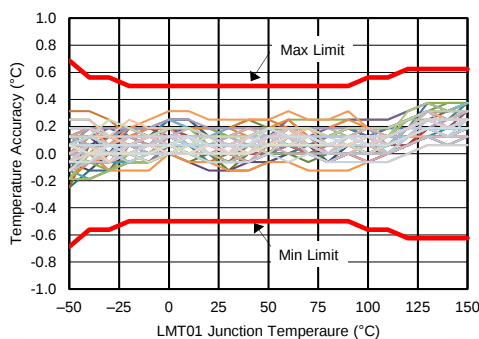
LMT01 Accuracy
