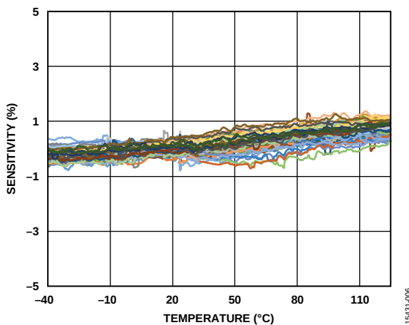
Figure 6. ADXL1001 Sensitivity vs. Temperature
