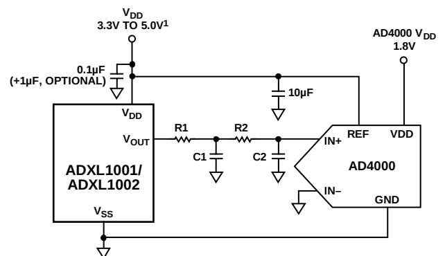
1.8V LIMITED BY ADXL1001/ADXL1002; 5.0V LIMITED BY AD4000
