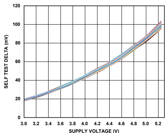
Figure 21. Typical Self Test Delta vs. Supply Voltage
