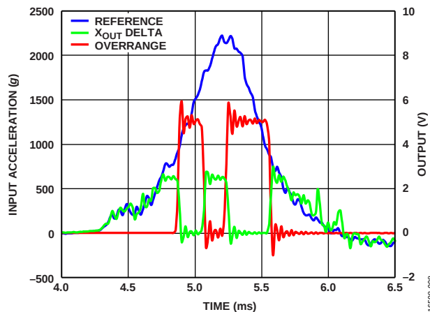
Figure 18. Response to Overload Condition, X_{OUT} Delta is Difference from Midscale Voltage
