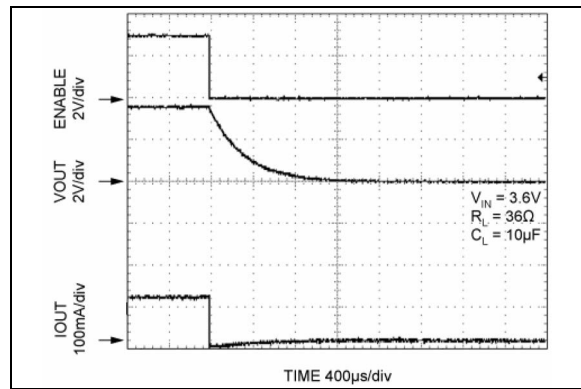
FIGURE 2-28: Turn-On/Turn-Off Timing.
