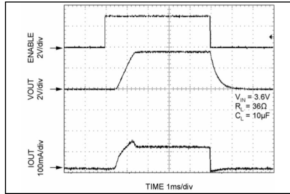
FIGURE 2-27: Turn-On/Turn-Off Timing.
