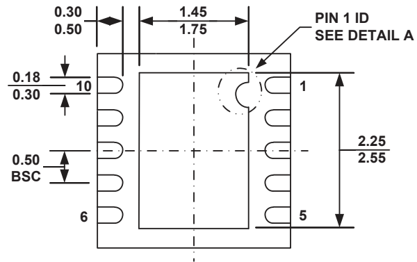
QFN10 (3 x 3mm)
