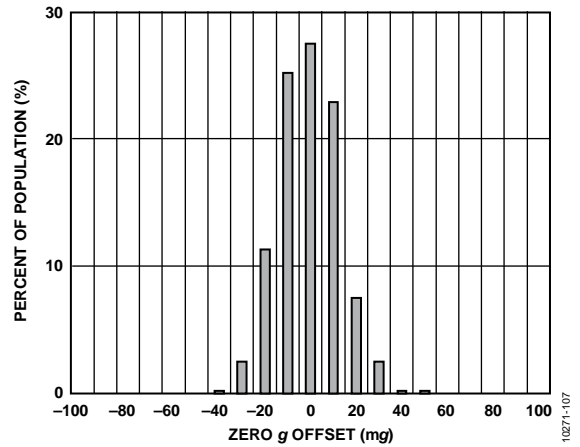
图8. 25°C时的Y轴0 g偏移, V_s = 3.0 V
