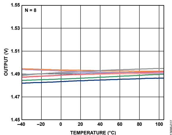
Figure 12. X-Axis Zero g Bias vs. Temperature
