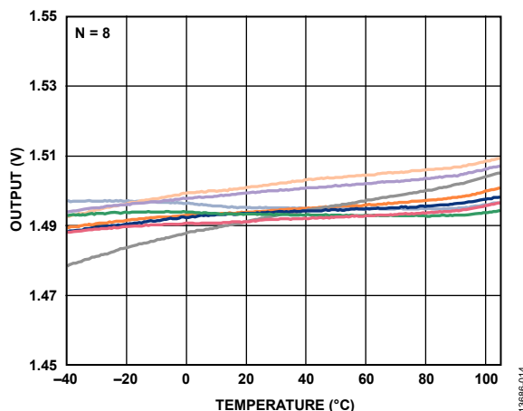
Figure 14. Z-Axis Zero g Bias vs. Temperature
