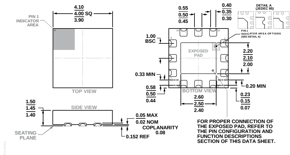
Figure 25. 12-Lead Lead Frame Chip Scale Package [LFCSP_SS] 4 mm × 4 mm Body and 1.45 mm Package Height, With Side Solderable Leads (CS-12-3) Dimensions shown in millimeters
