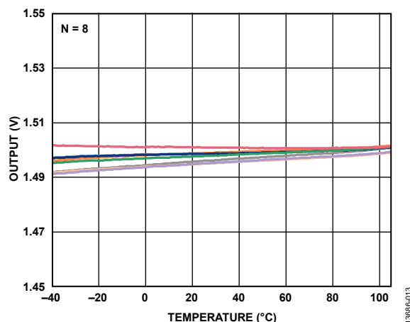
Figure 13. Y-Axis Zero g Bias vs. Temperature
