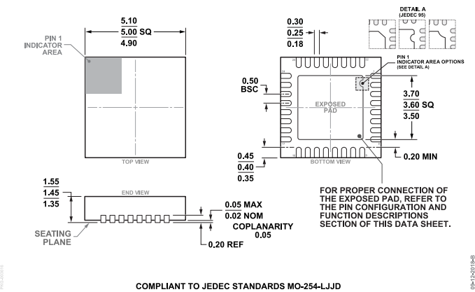
Figure 30. 32-Lead Lead Frame Chip Scale Package [LFCSP] 5 mm x 5 mm Body, Thick Quad (CP-32-17) Dimensions shown in millimeters
