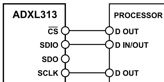
Figure 16. 3-Wire SPI Connection Diagram
