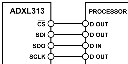
Figure 17. 4-Wire SPI Connection Diagram
