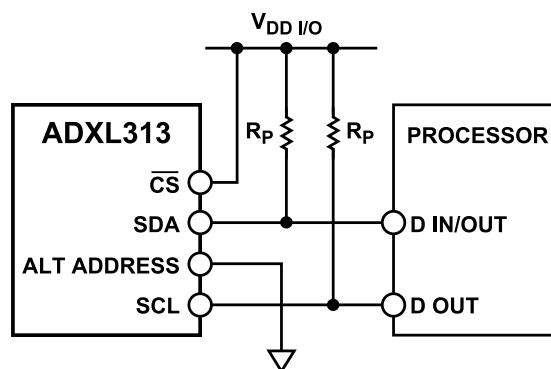
Figure 21. I 2 C Connection Diagram (Address 0x53)
