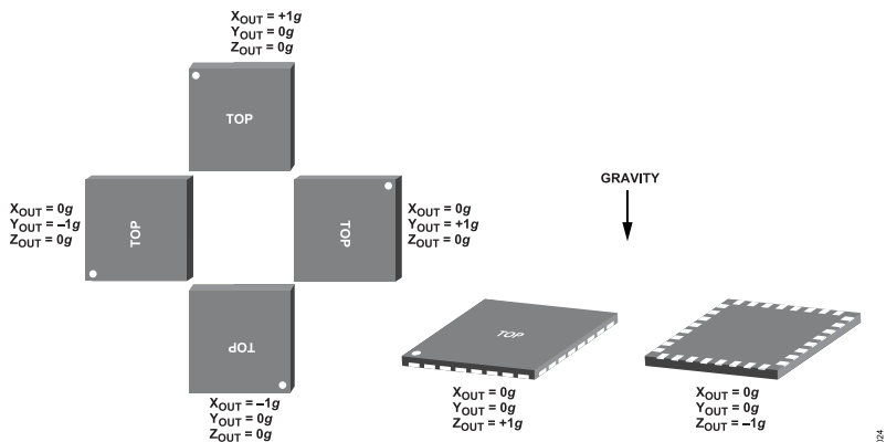
Figure 29. Output Response vs. Orientation to Gravity
