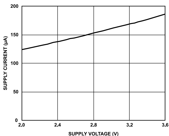
Figure 15. Supply Current vs. Supply Voltage, V_S at 25^\circ\text{C}
