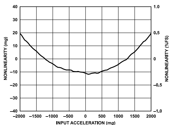
Figure 9. Z-Axis Nonlinearity, \pm 2 g Input Range
