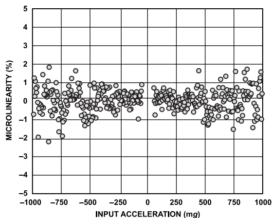
Figure 11. Y-Axis Microlinearity, 50 mg Step Size
