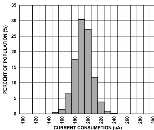
Figure 14. Current Consumption, Measurement Mode, Data Rate = 100 Hz, V_S = V_{DD I/O} = 3.3\text{ V} , 25^\circ\text{C}
