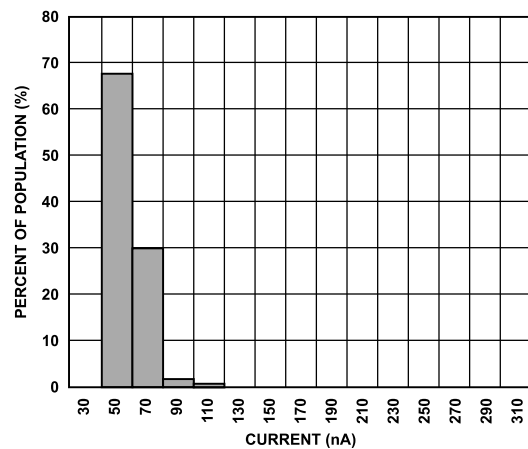
Figure 13. Standby Mode Current Consumption, V_S = V_{DD I/O} = 3.3\text{ V} , 25^\circ\text{C}
