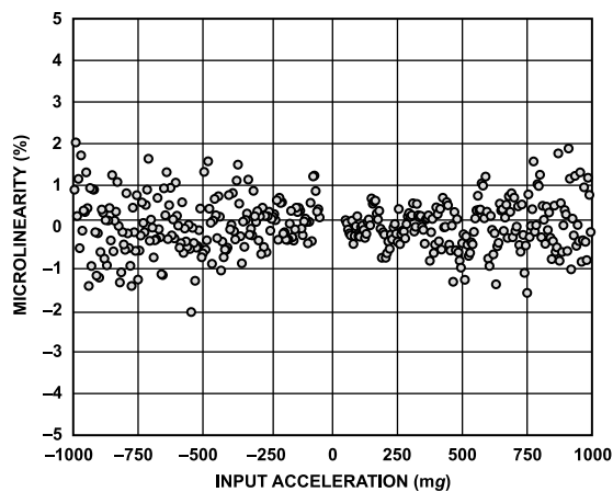
Figure 10. X-Axis Microlinearity, 50 mg Step Size
