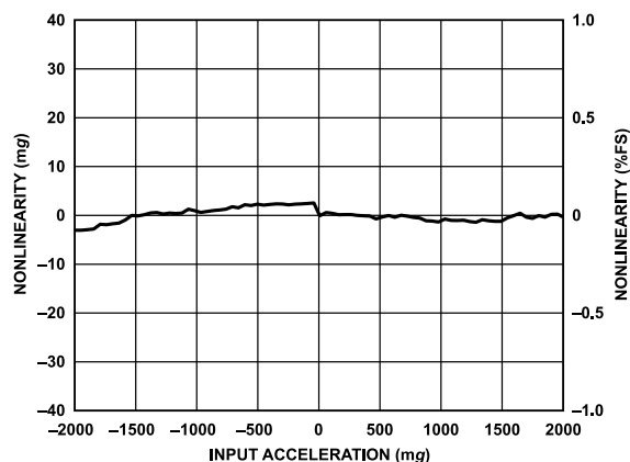
Figure 7. X-Axis Nonlinearity, \pm 2 g Input Range
