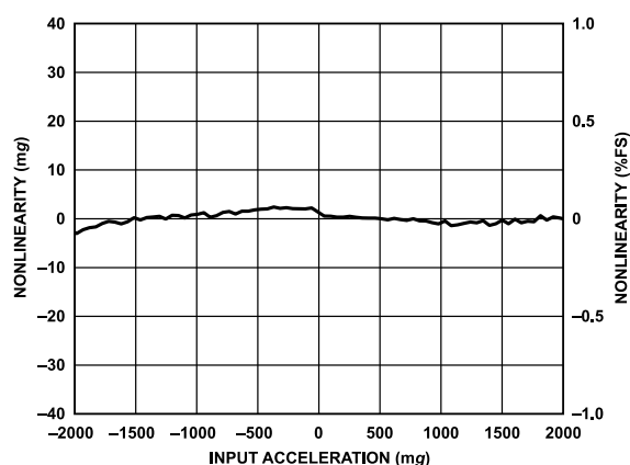
Figure 8. Y-Axis Nonlinearity, \pm 2 g Input Range
