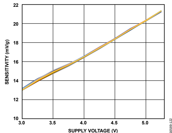
Figure 22. Sensitivity vs. Supply Voltage
