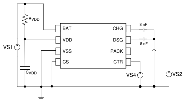
Figure 9-4. Test Circuit 4
