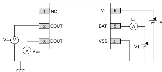
Figure 8-4. Test Circuit 2
