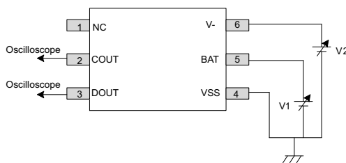
Figure 8-7. Test Circuit 5
