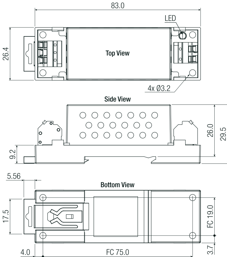
Dimension Drawing "/PMAD-CTN" version (mm)
