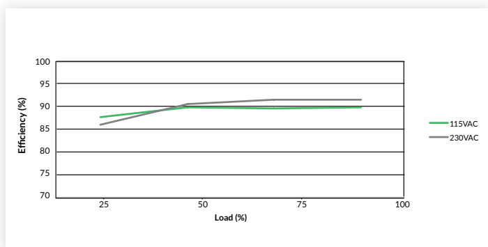
Figure 4 SMP350PS48
