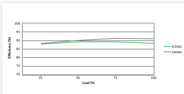
Figure 3 SMP350PS24
