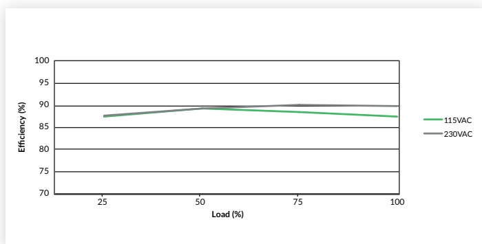
Figure 2 SMP350PS12
