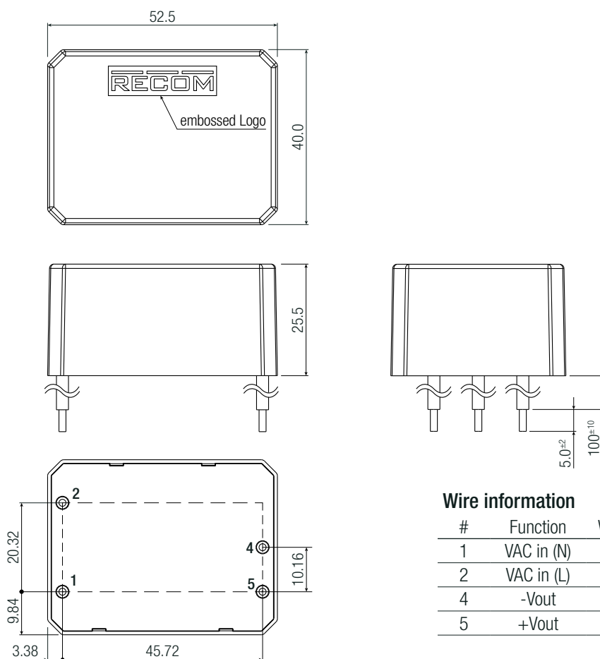
Dimension Drawing Wired version "/W" SINGLE Output (mm)
