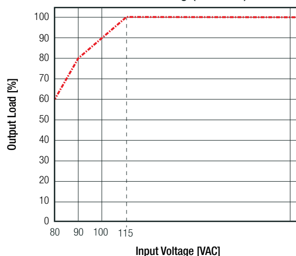
Line Derating (<115VAC)
