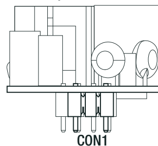
AC Input Side View
