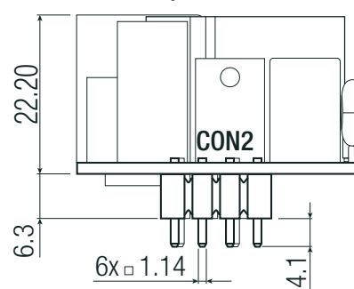
DC Output Side View
