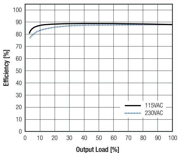
RACM40-05SK/OF
