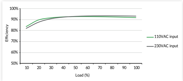
Figure 1 - UCH600PS12
