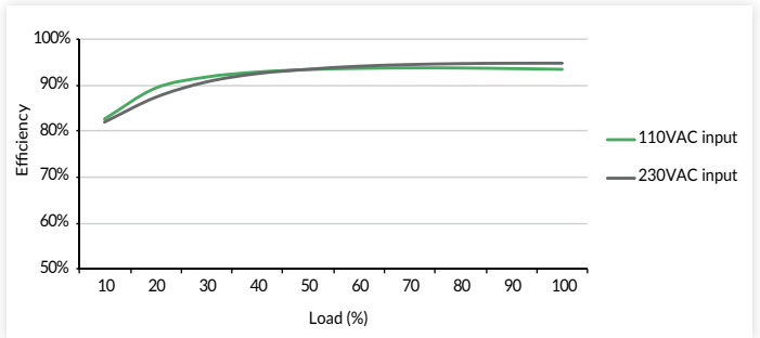
Figure 2 - UCH600PS24
